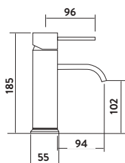
Mono Basin Mixer
