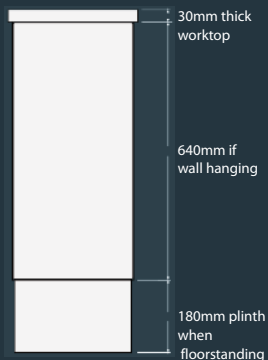
Base Unit Dimensions
