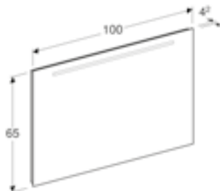
100cm mirror with functional lighting from the top W 100 / D 4.2 / H 65cm Mechanical switch, LED lighting. Art. no. 500.584.00.1
