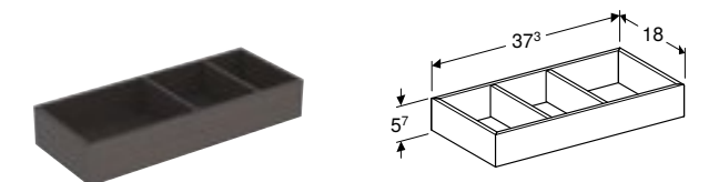
Square drawer insert low W 18 / D 37.3 / H 5.7cm
