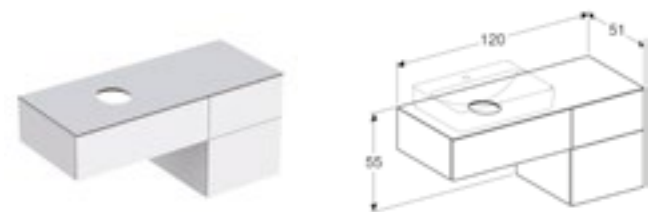
120cm cabinet for lay-on washbasin, with three drawers W 120 / D 51 / H 55cm
