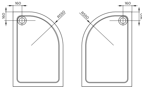
OFFSET QUADRANT RIGHT HAND
