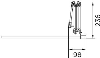
AQ9357LS/RS Swiftseal Semi Frameless 4 Fold Bath Screen Available as left or right hand option
