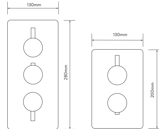
CONTROLLERS
