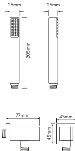
HAND SHOWER AND HOLDER
