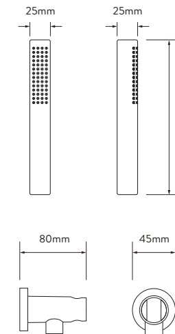
HAND SHOWER AND HOLDER
