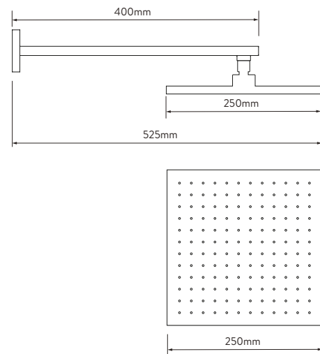
FIXED HEAD
