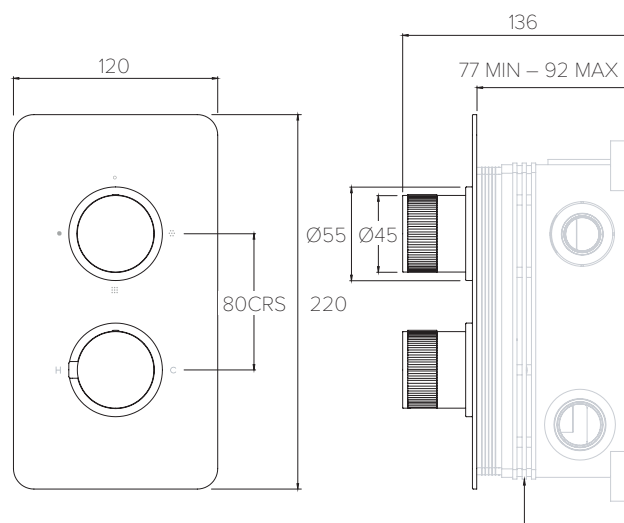
SEE DRAWING: CO3002 – 2 OUTLET C-BOX
