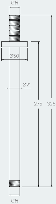
300mm CEILING ARM
