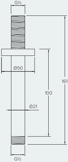
100mm CEILING ARM
